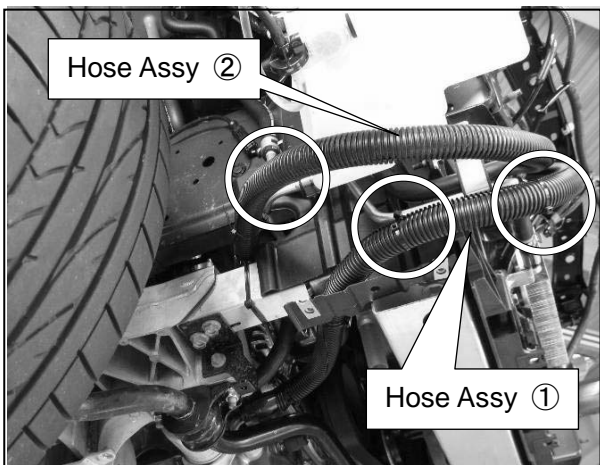
Secure the hoses to the P/S cooler piping using the provided Tie Wraps.
