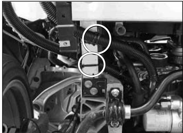
Secure the Hose Assy to the side member.
