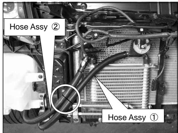
Bundle the hoses using the provided Tie Wraps.
